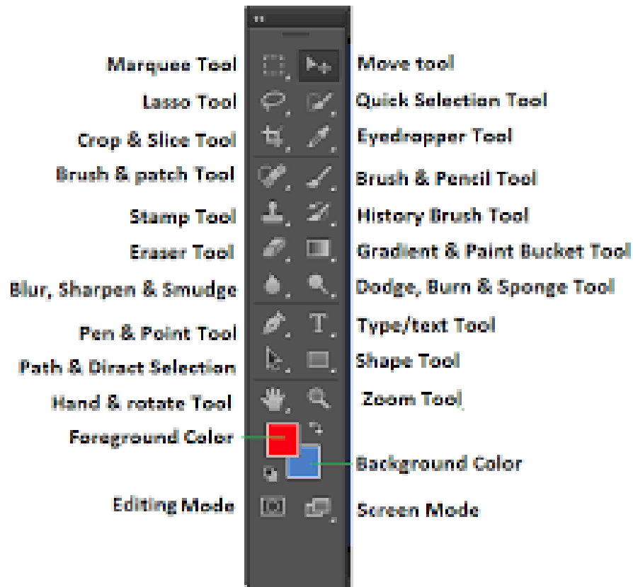
Image 2: Toolbox
