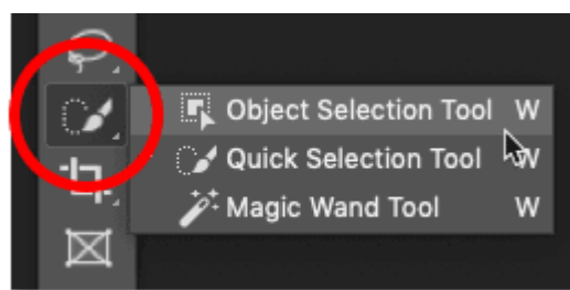
Image 1: Selection Tools
