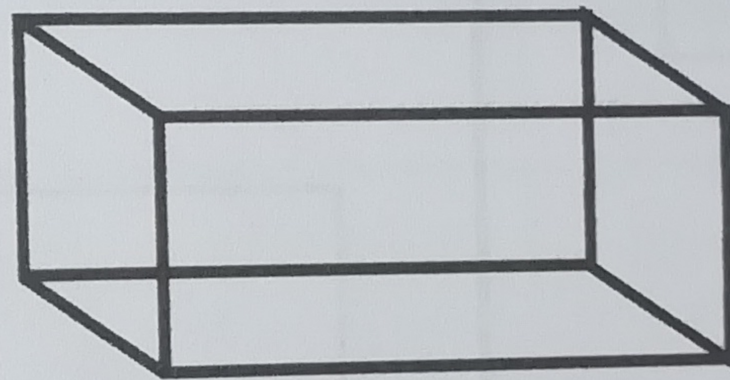
Cuboid
