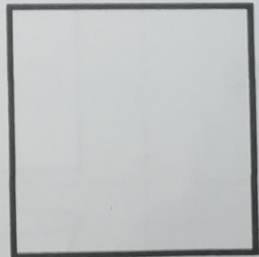
Square
