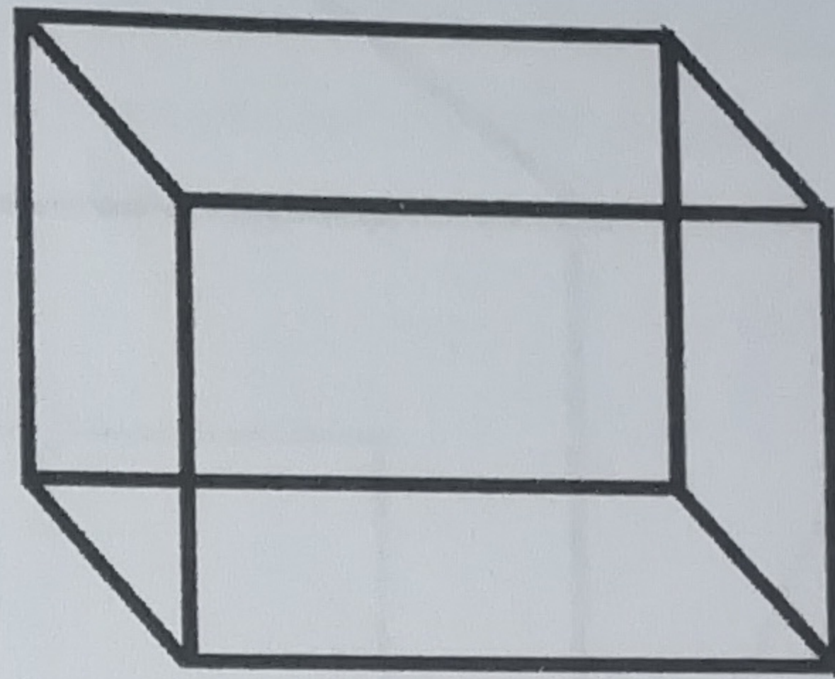
Cube
