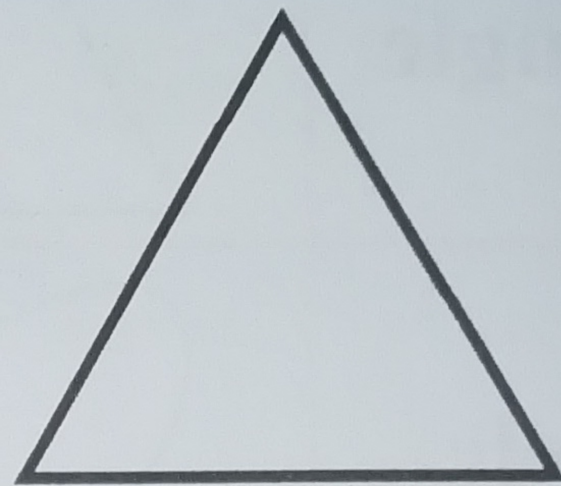
Triangle
