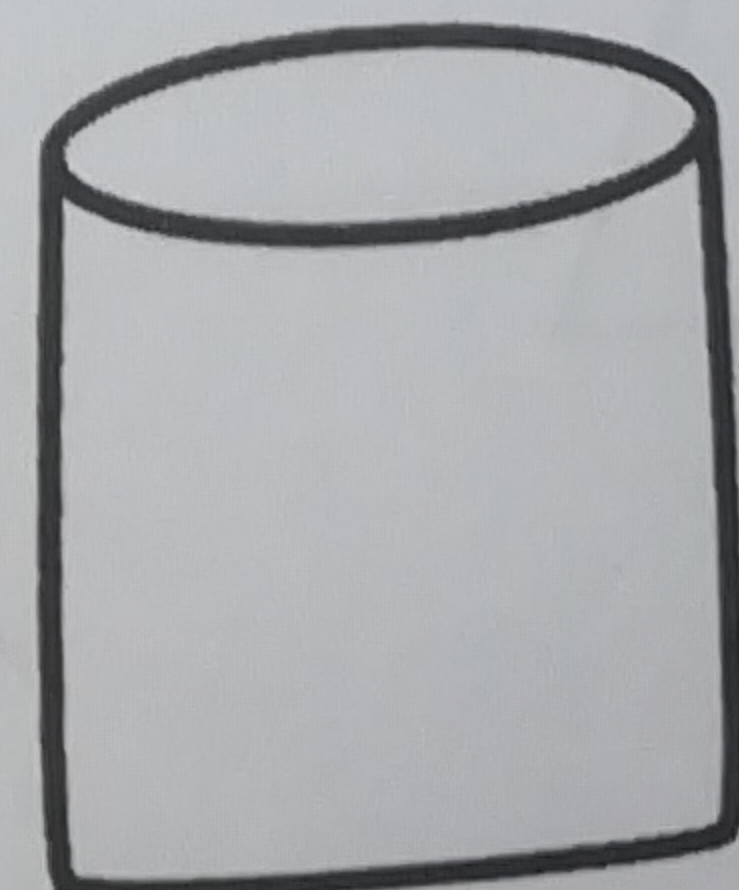
Cylinder
